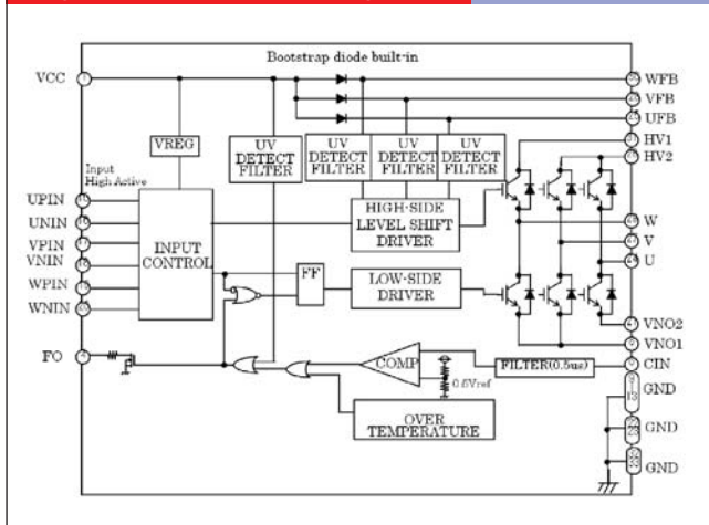
Single Chip Inverter Block Diagram
