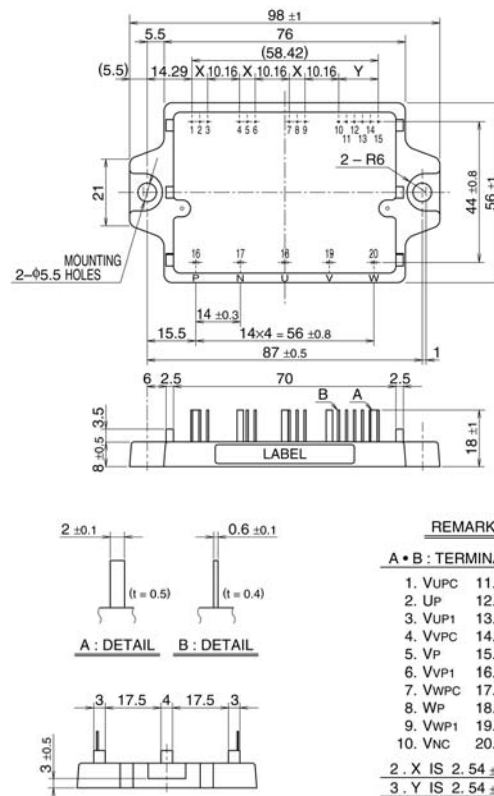
Package S16
