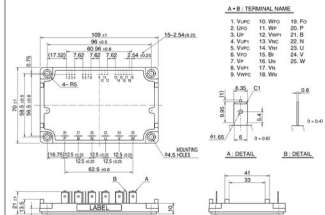
Package S12
