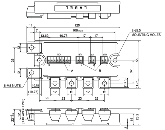
Package NF4
