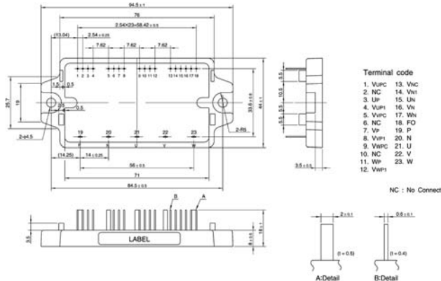
Package S6
