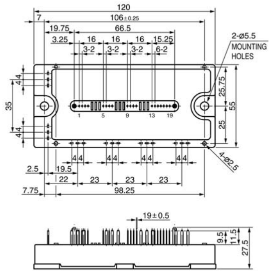
Package L2
