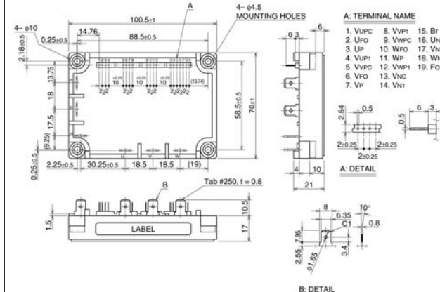
Package S11
