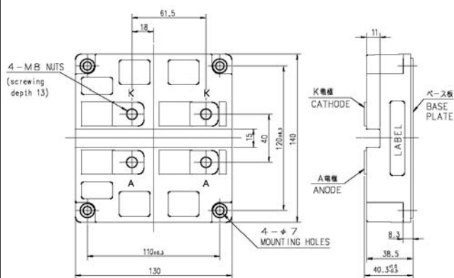
Package RM5
