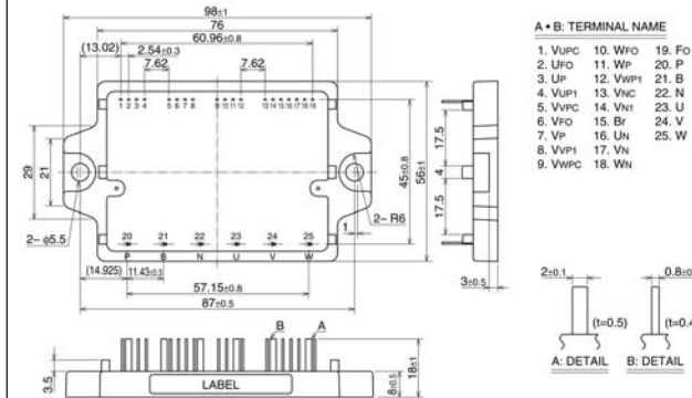
Package S9
