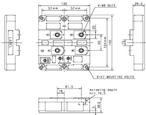
Package RM3
