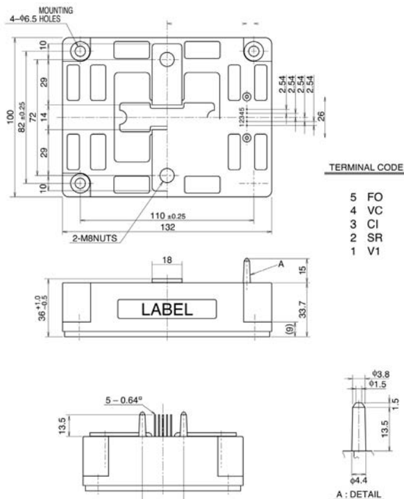
Package S15
