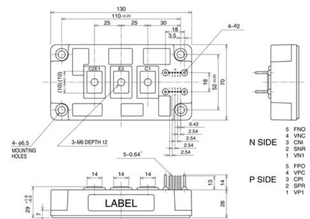
Package S4
