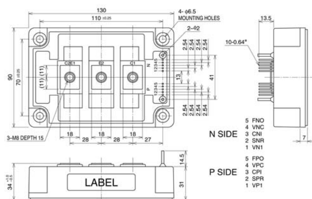
Package S5
