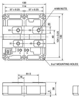
Package RM1
