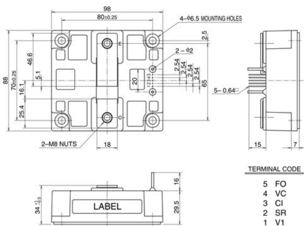
Package S1
