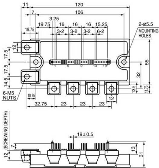
Package L1
