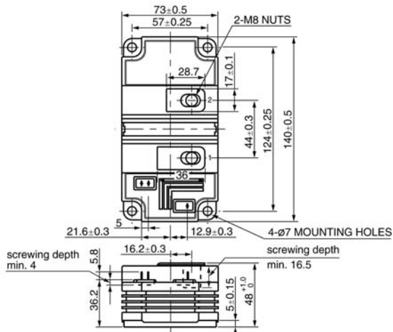
Package HV9
