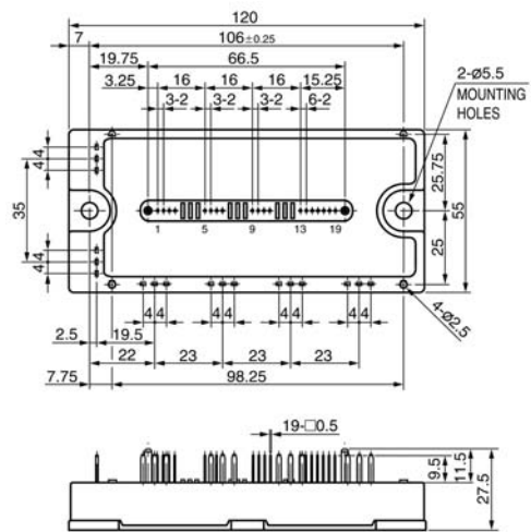
Package L2
