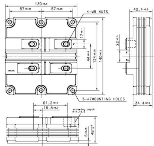
Package RM4
