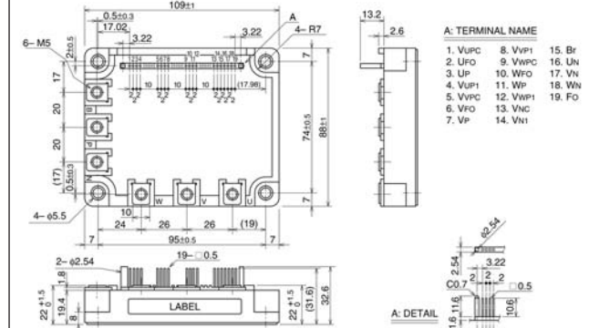
Package S10
