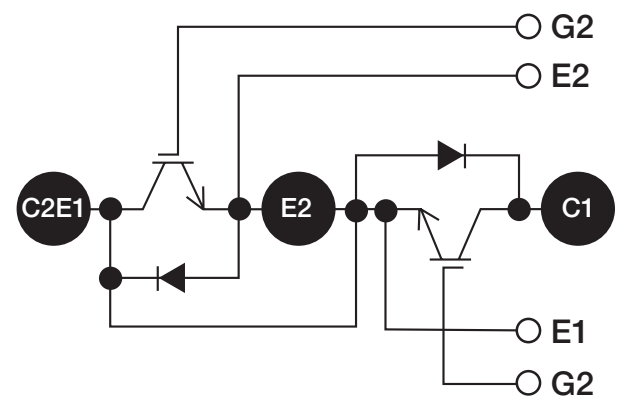
Circuit Diagram
