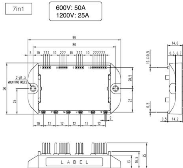
Package L5
