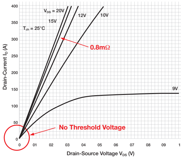
Example FM400TU-07A
