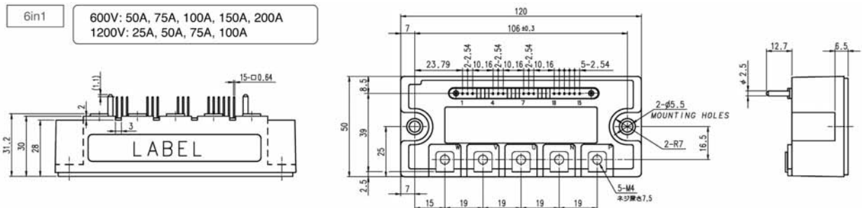
Package S1
