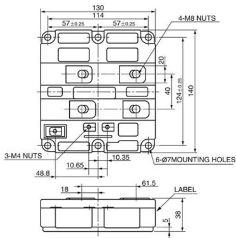
Package HV7
