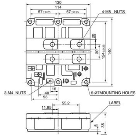
Package HV4
