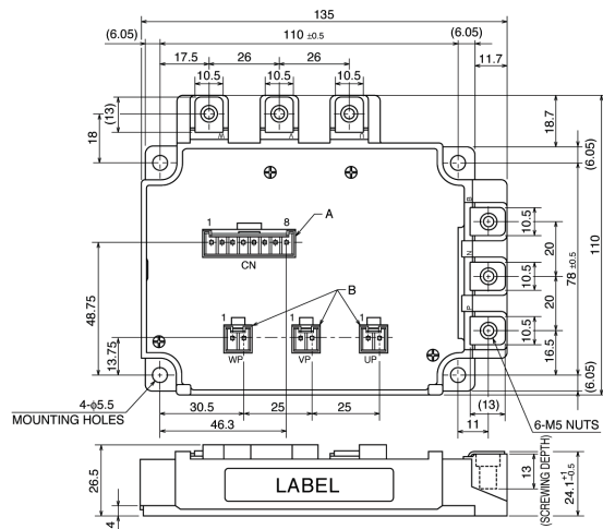
Package NF5
