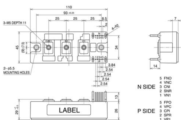
Package S2
