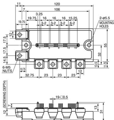
Package L1
