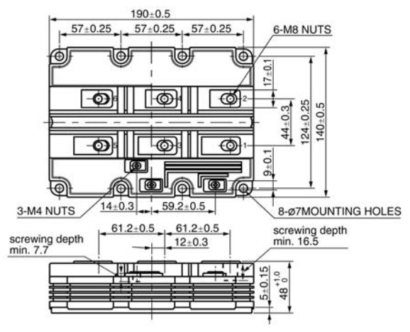
Package HV8
