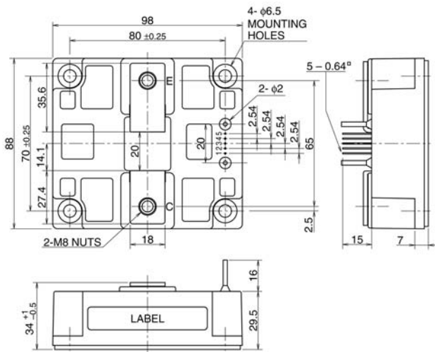
Package S13
