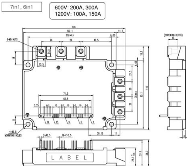
Package L3
