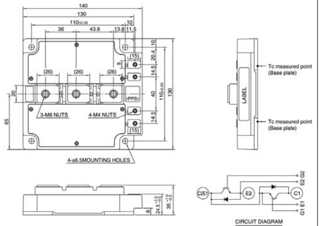
Package NF6
