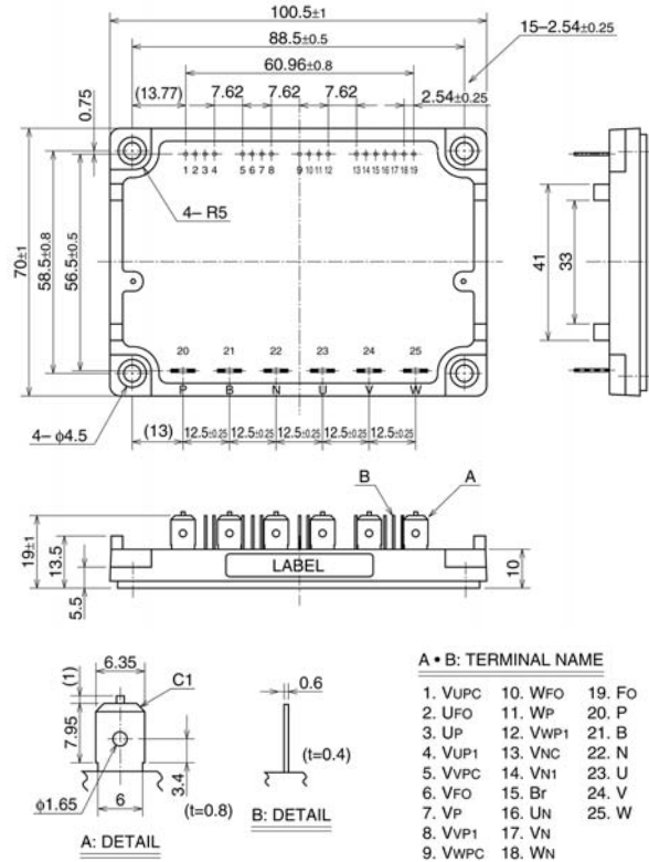
Package S19
