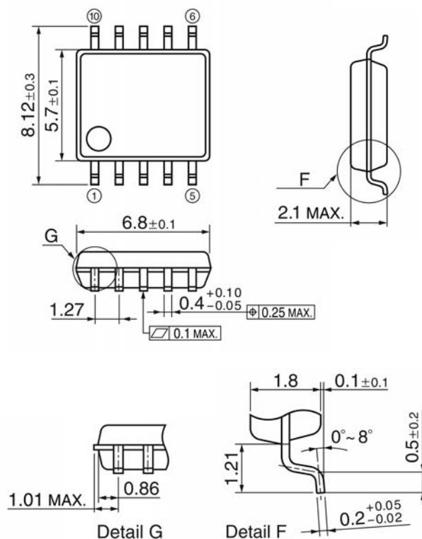
Package 10P2N (10pin 300mil SOP)
